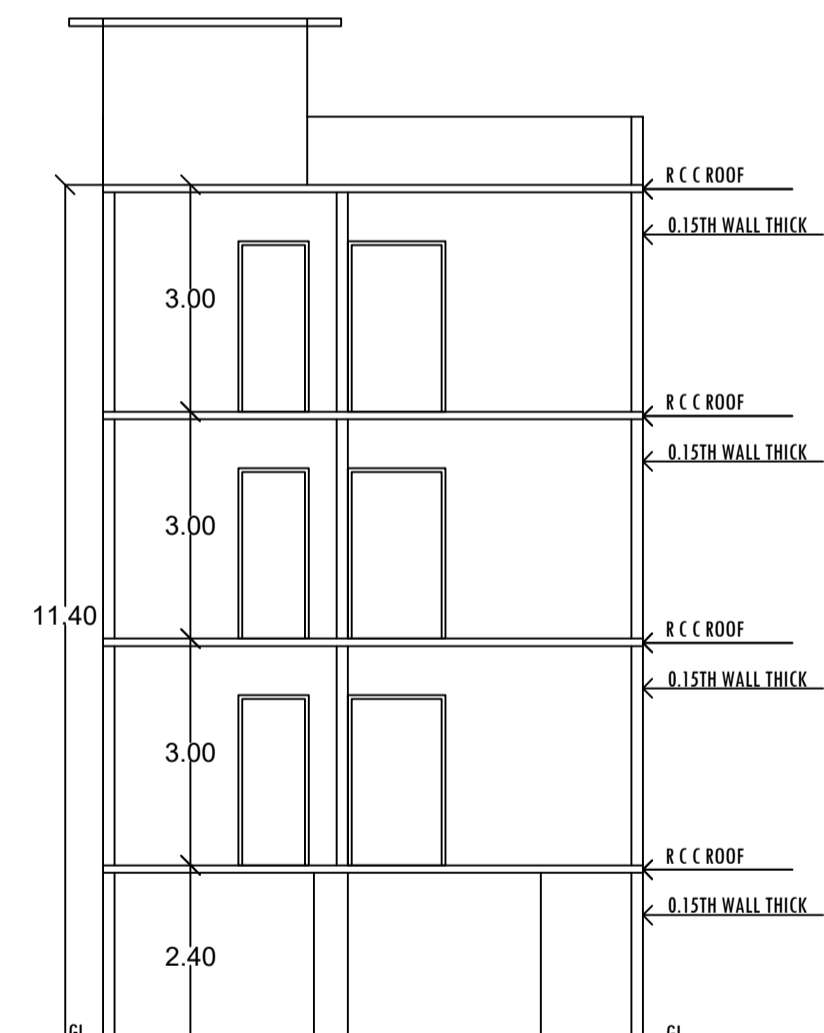
SECTION X-X
